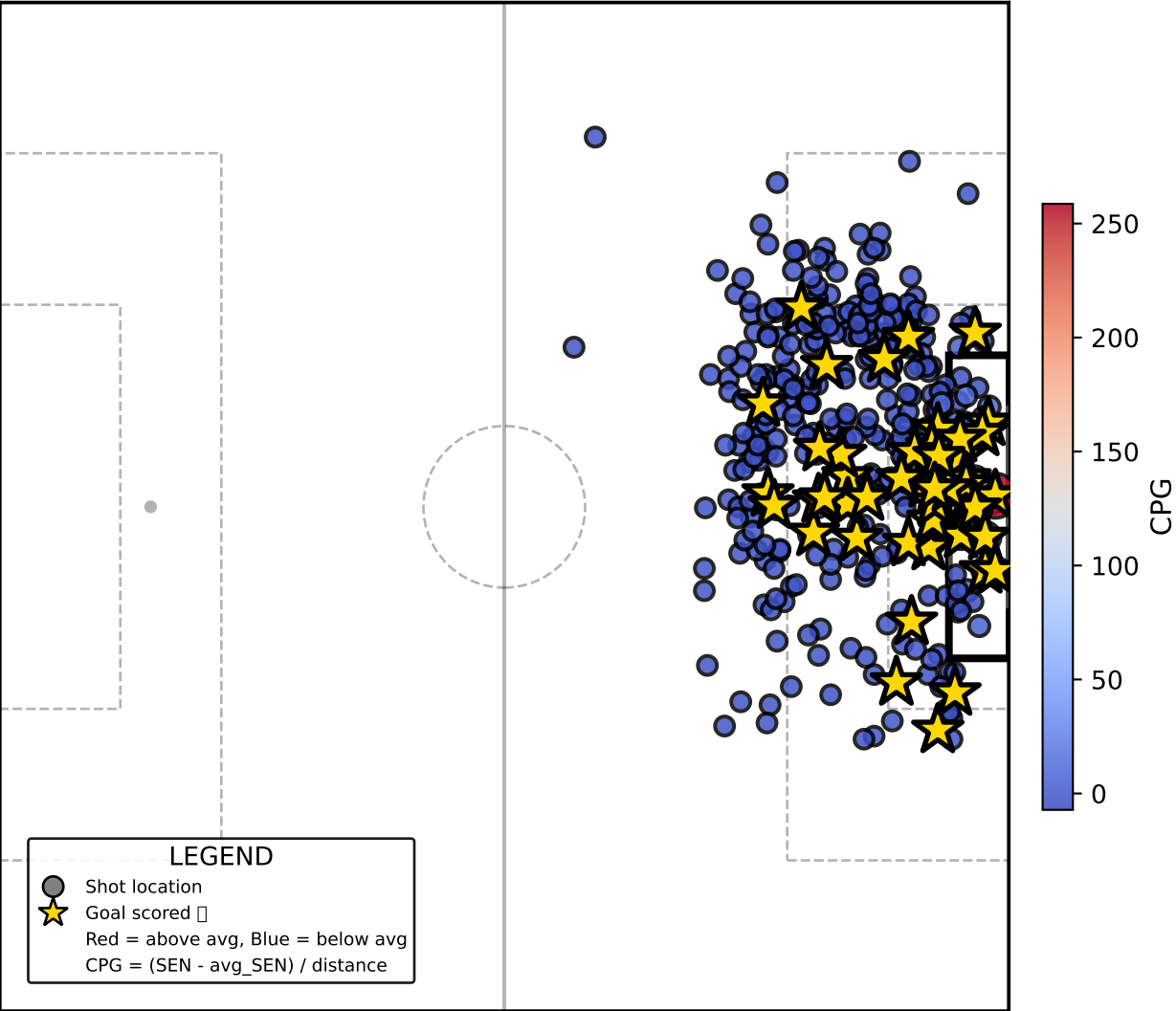
Conversion Pressure Gradient (CPG) Alexis Sánchez | 463 shots, 63 goals
