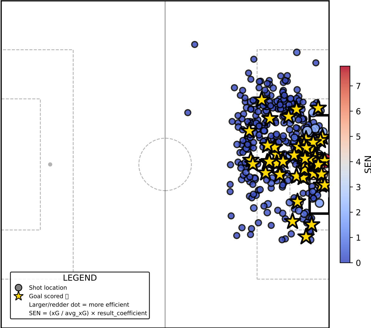
Shot Efficiency Number (SEN) Alexis Sánchez | 463 shots, 63 goals
